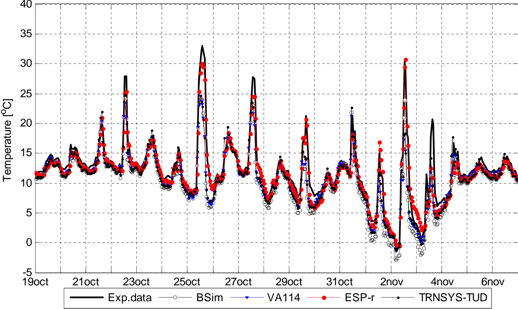
Hour averaged temperature of the external window glass surface facing zone1
